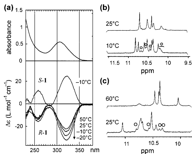
Figure 3. (a) Electronic absorption and CD spectra of 1 M solutions of ( S )- and ( R )- 1 in \text{CHCl}_3 at various temperatures. Spectra could not be measured below 210 nm because the oligomers are not soluble in solvents that do not absorb at these wavelengths. Part of the ^1\text{H} NMR (400 MHz) spectra of ( R )- 1 showing the amide resonances in (b) \text{CDCl}_3 and (c) [\text{D}_8]\text{toluene} . The circles indicate signals from the minor helical diastereomer.
